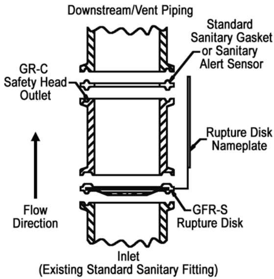
Figure 1 GR-C Safety Head with GFR-S Rupture Disk
