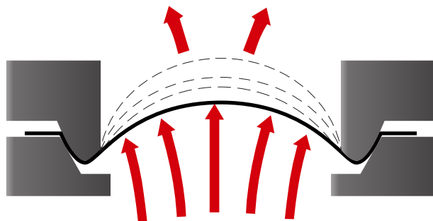
Example: Cross-section diagram of a Type B tension loaded conventional rupture disk and FA-7R Quik-Sert safety head. With 30-degree angular seating, pressure loading is on concave side of disk. This puts the disk metal under tension. As pressure increases on a conventional disk in tension, the seating design allows the dome to thin out to a point where it can no longer withstand the pressure. The disk ruptures and metal segments fold back against the walls of the fitting in an irregular pattern to provide a full opening.
